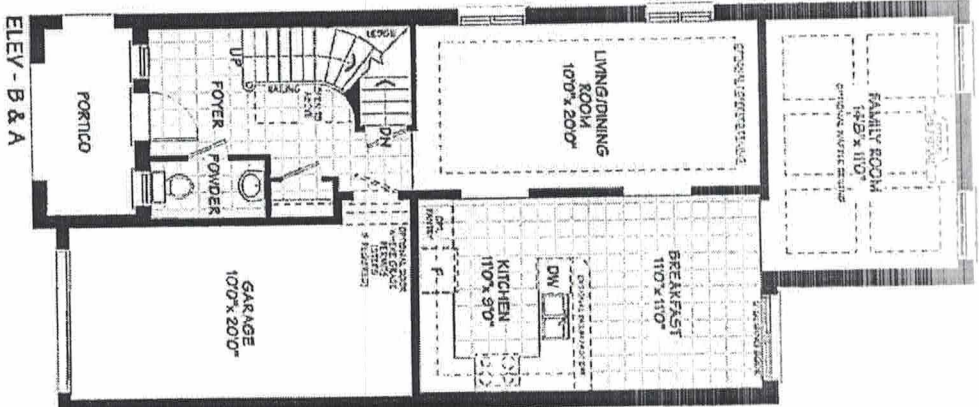
MAIN FLOOR
