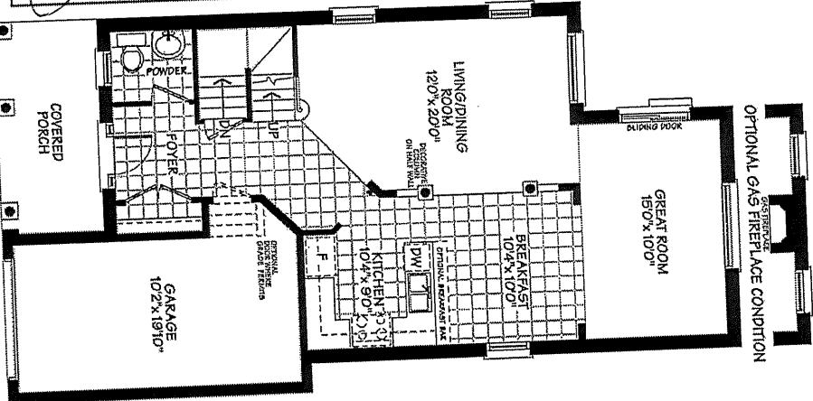
Elevation A - 1658 sq. ft.
