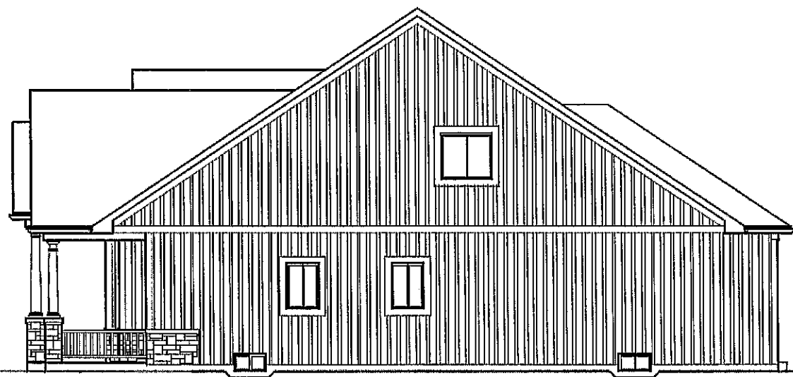
RIGHT SIDE ELEVATION 'A'
