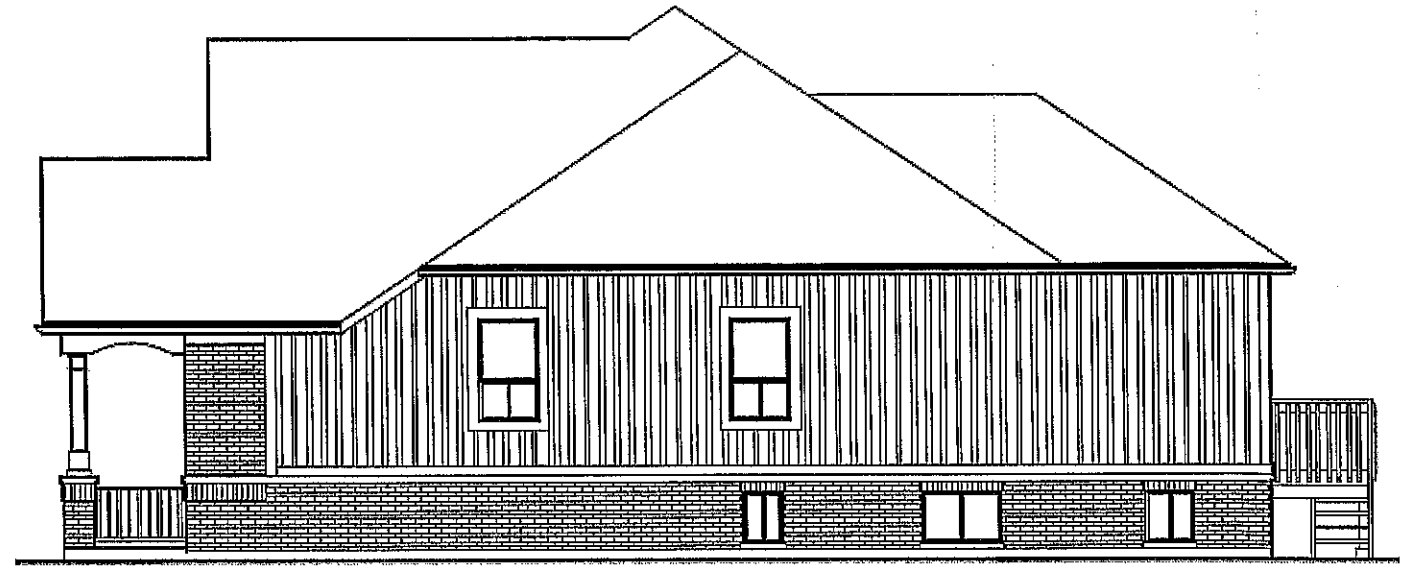
RIGHT SIDE ELEVATION 'B'
