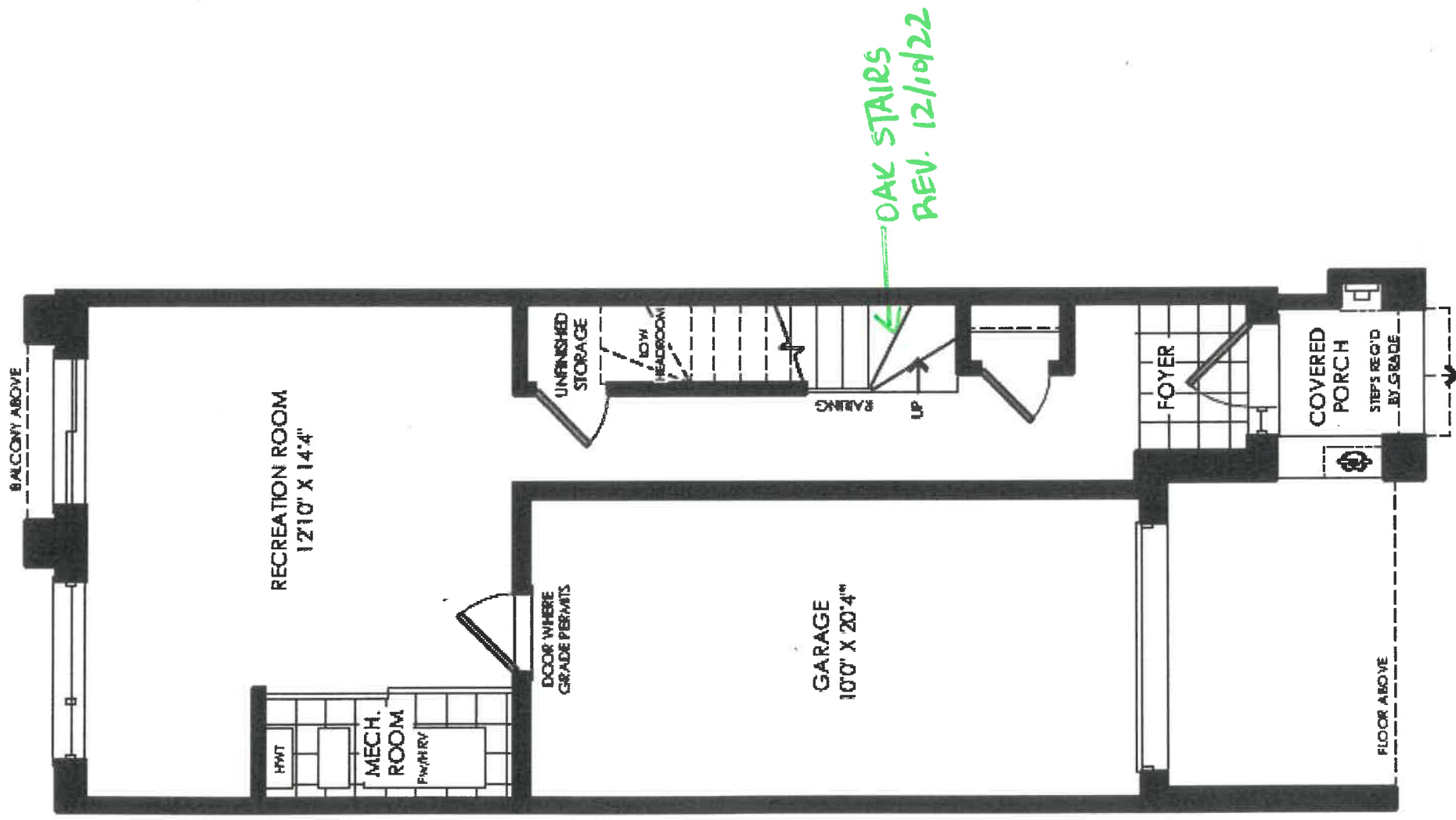
GROUND FLOOR ELEV. 'A'
