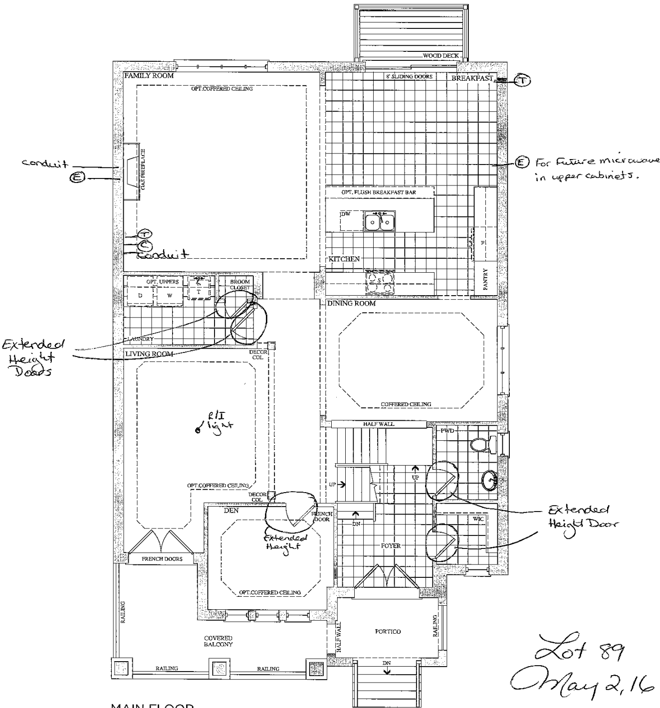
MAIN FLOOR ELEVATION A
