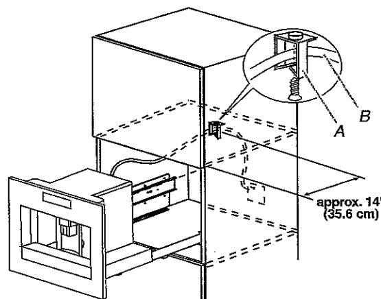
A. Power supply cord clip
