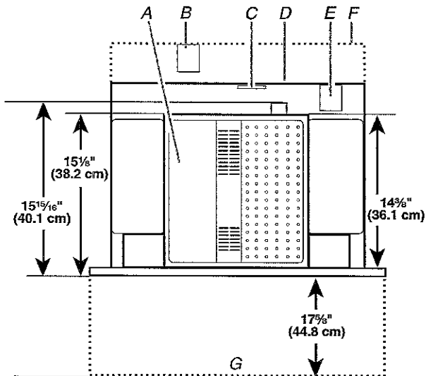
Cutout Top View
