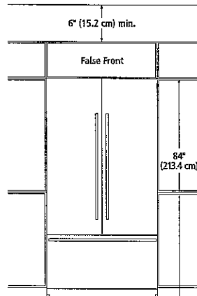
FRONT VIEW – FALSE FRONT (OPTION 2)
