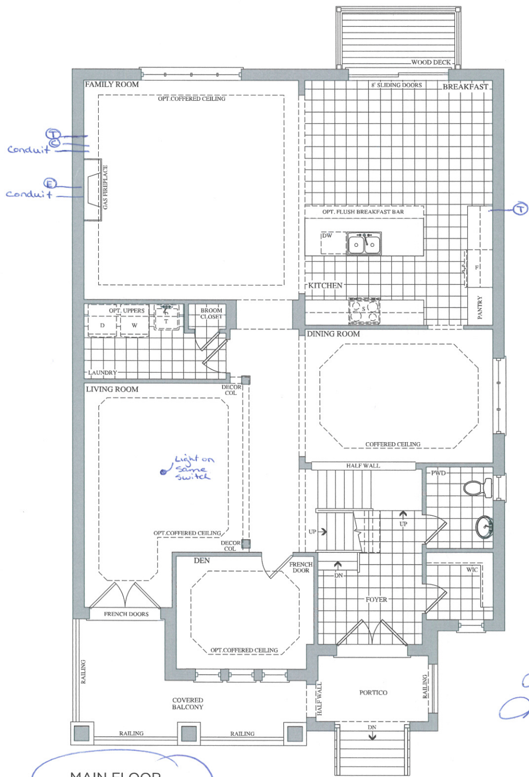
MAIN FLOOR ELEVATION A
