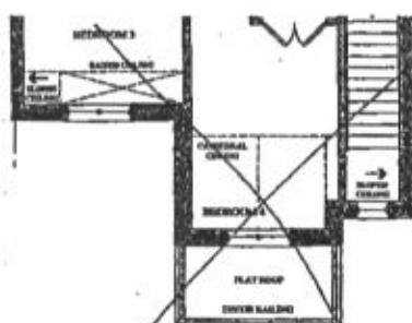
PART. OPT. 4 BED SECOND FLOOR PLAN
