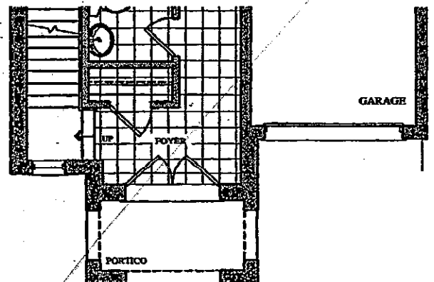
PART. GROUND FLOOR PLAN ELEV. 'C' & 'D'
