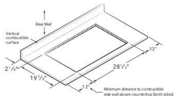
Cutout Dimensions of Countertop
