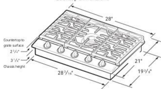
Cooktop Dimensions
