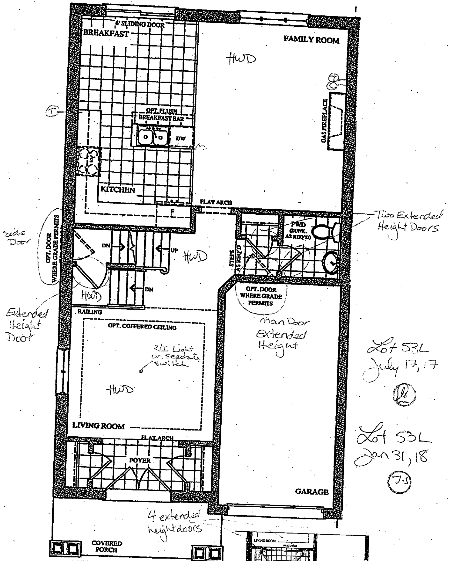
GROUND FLOOR PLAN ELEV. 'A' & 'B'
