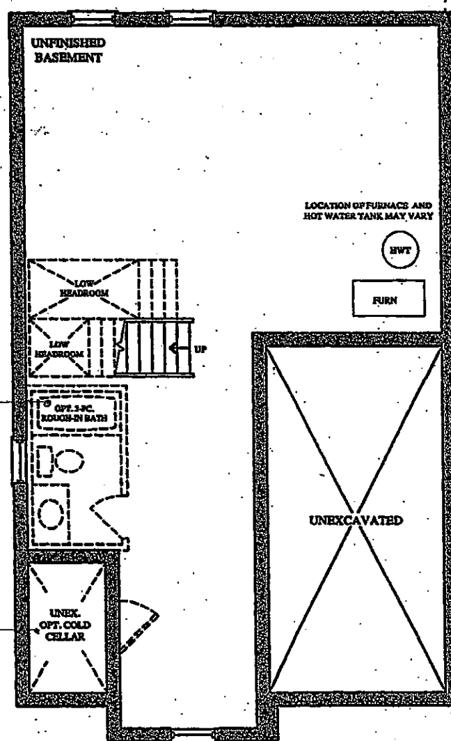
BASEMENT FLOOR PLAN ELEV. 'A', 'B' & 'C'
