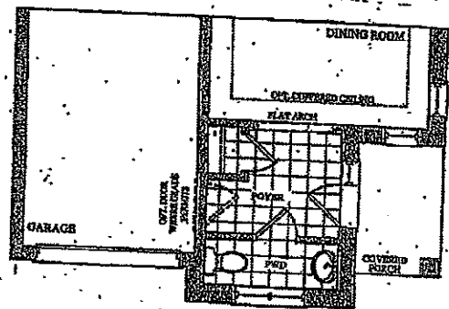
PART. GROUND FLOOR PLAN ELEV. 'C'
