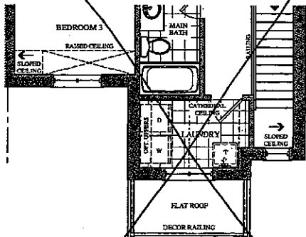
PART. SECOND FLOOR PLAN ELEV. 'D'
