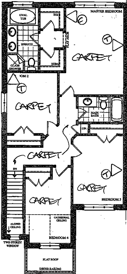
* OPT. 4 BED SECOND FLOOR PLAN ELEV. 'A'
