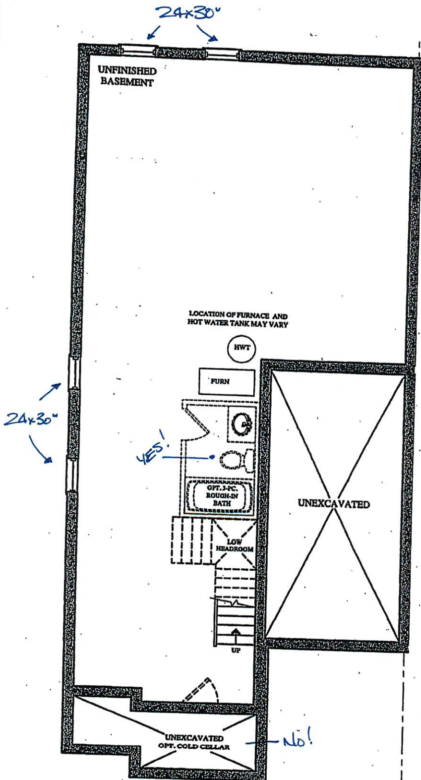
BASEMENT FLOOR PLAN ELEV. 'A' & 'B'
