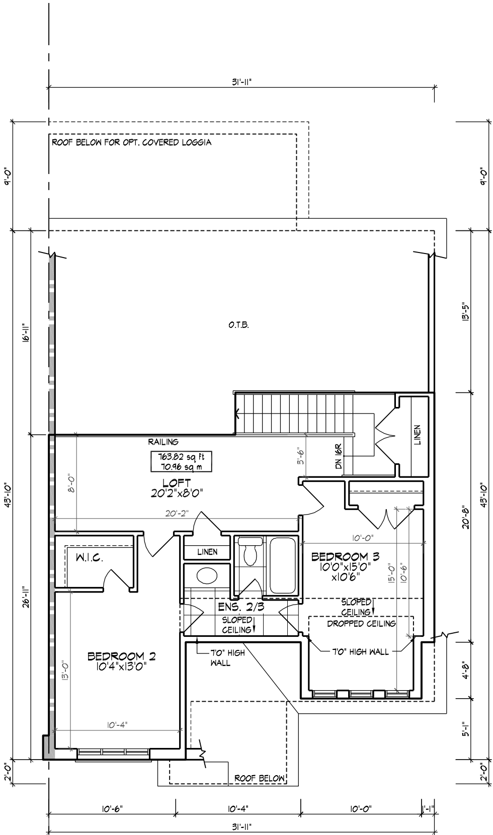
LOFT PLAN, EL. 'A' - 3105
