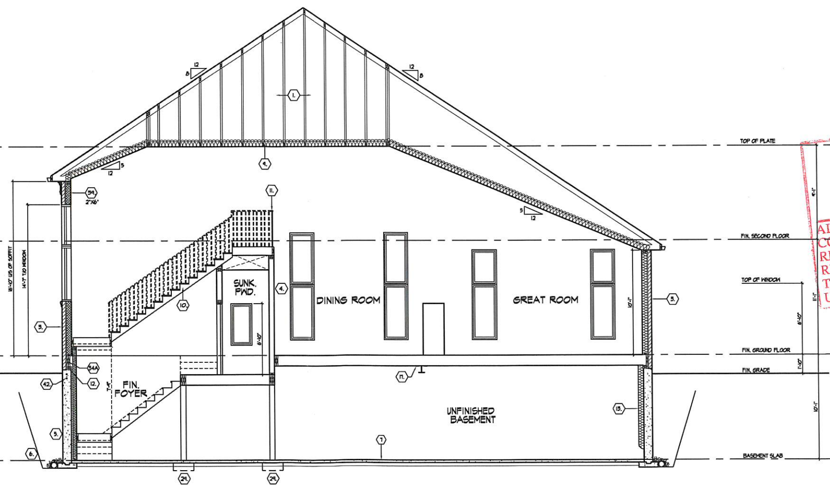
CROSS SECTION 'A-A'
