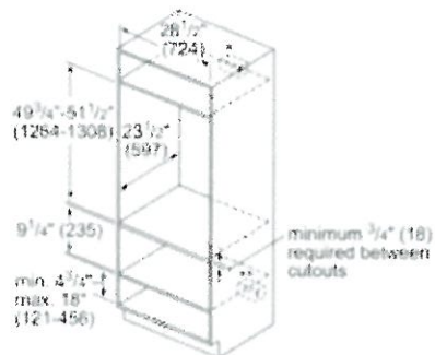
Standard Installation 30" Double Oven over Storage or Warming Drawer
