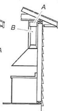
Non-Vented (Recirculating)
