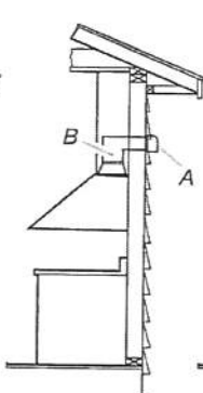
Wall Venting
