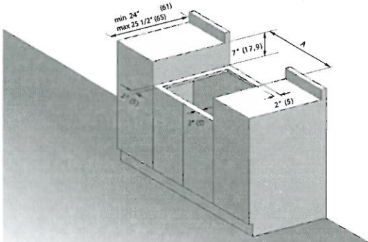
INSTALLATION WITHOUT SEPARATOR SHEET
