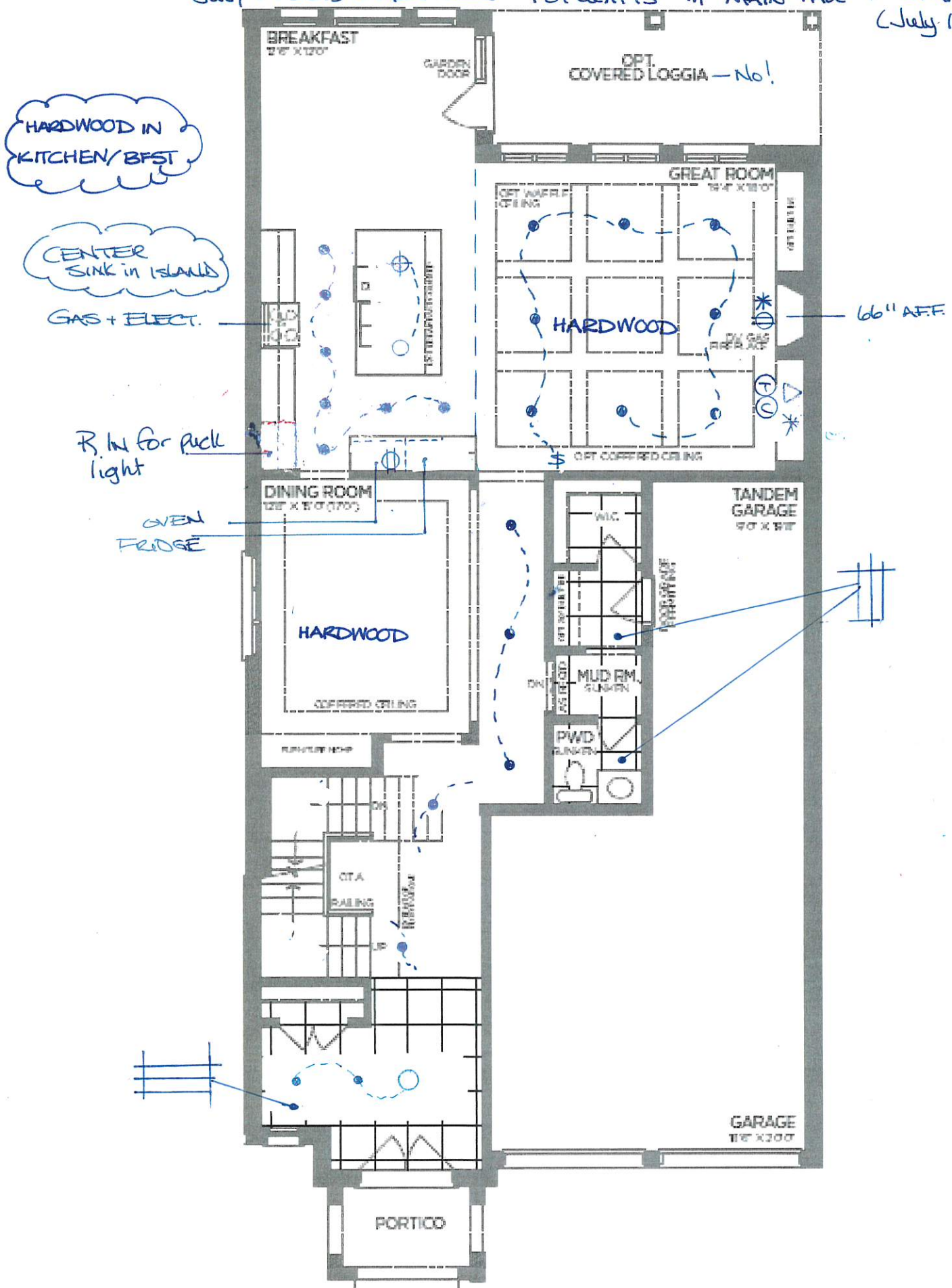
GROUND FLOOR | ELEV. A
