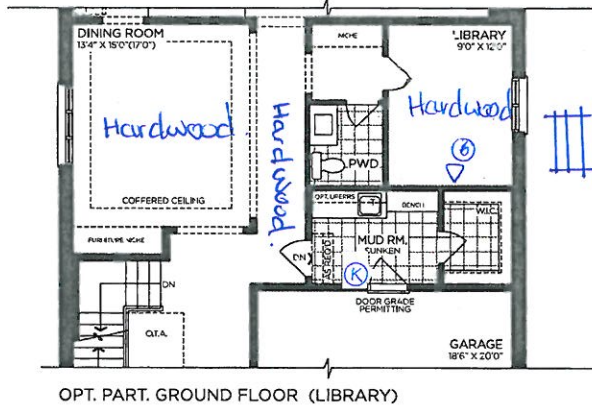
OPT. PART. GROUND FLOOR (LIBRARY)
