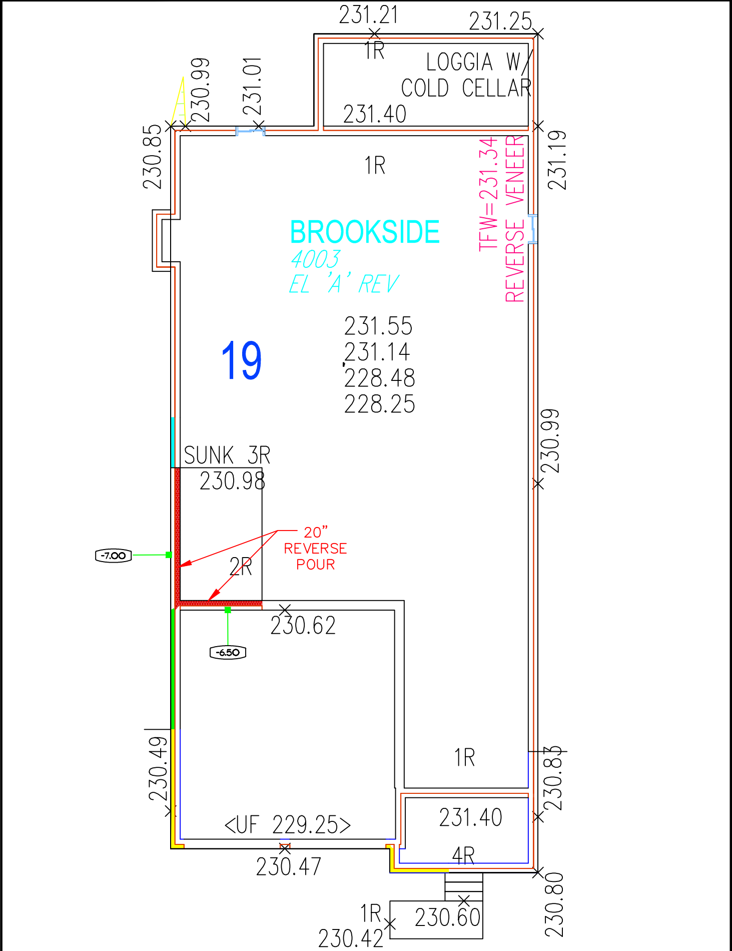
PLAN
