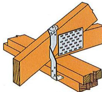
MTS Installation as a Truss-to-Top Plate Tie
