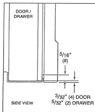
Door/Drawer Bottom
