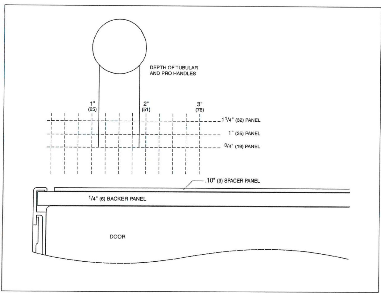
Overlay and flush inset panel thickness.
