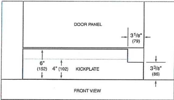
Kickplate notch
