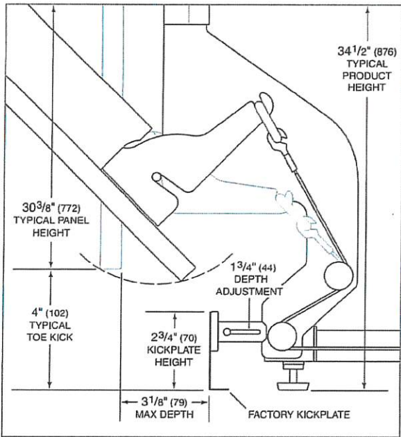
Toe kick area (side view)
