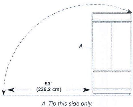
Side Tipping Radius (42" [106.7 cm] Models)
