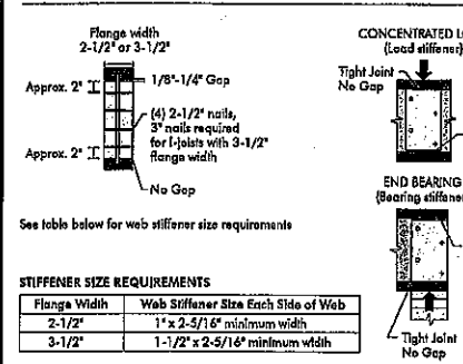
FIGURE 2 WEB STIFFENER INSTALLATION DETAILS
