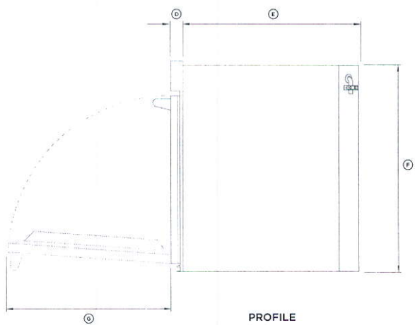
PROFILE
