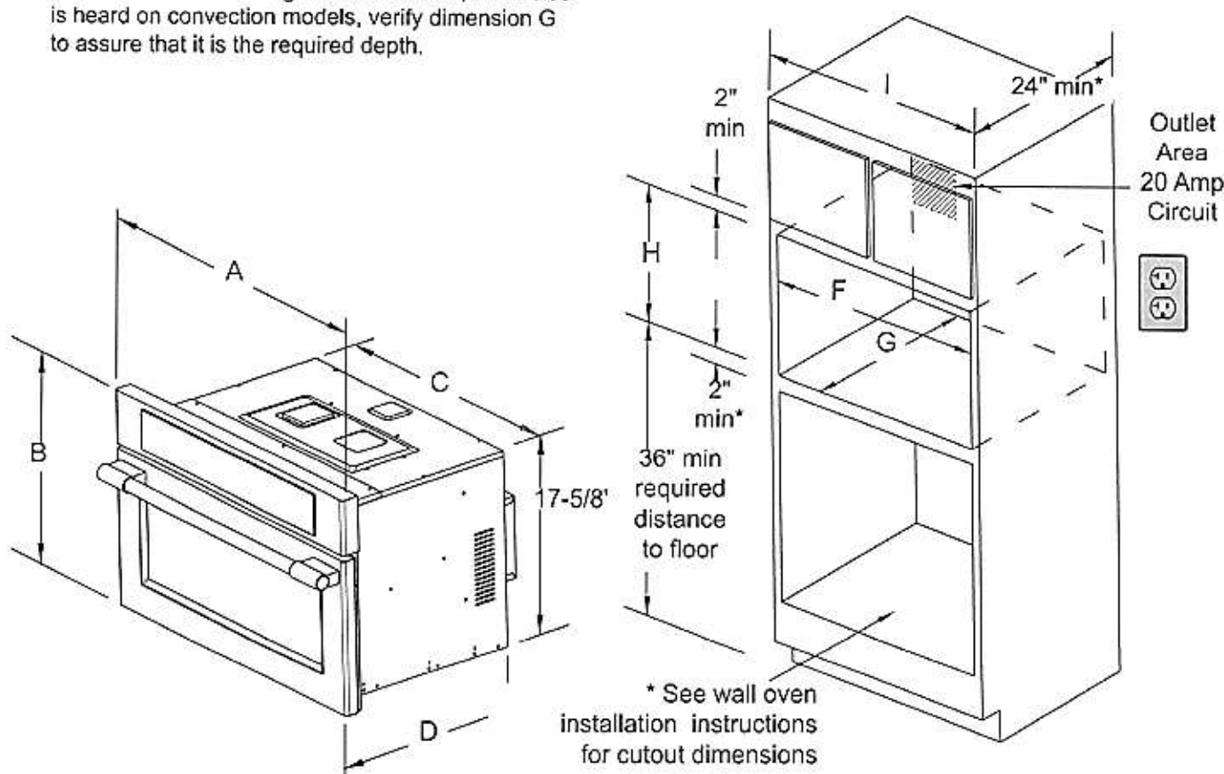
Figure 3: Microwave with Wall Oven
