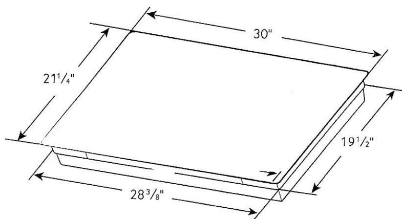
Cooktop Dimensions
