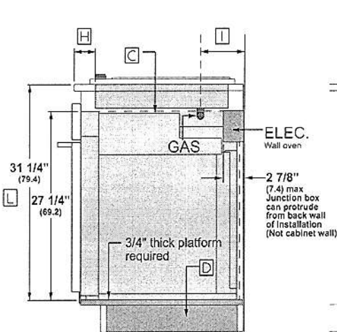
STANDARD INSTALLATION SIDE VIEW
