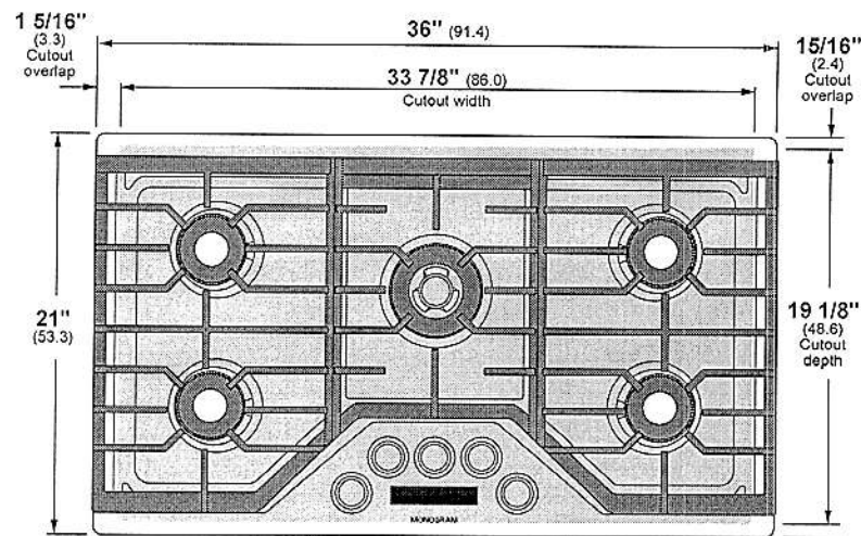
TOP VIEW (SHOWING CUTOUT OVERLAP)
