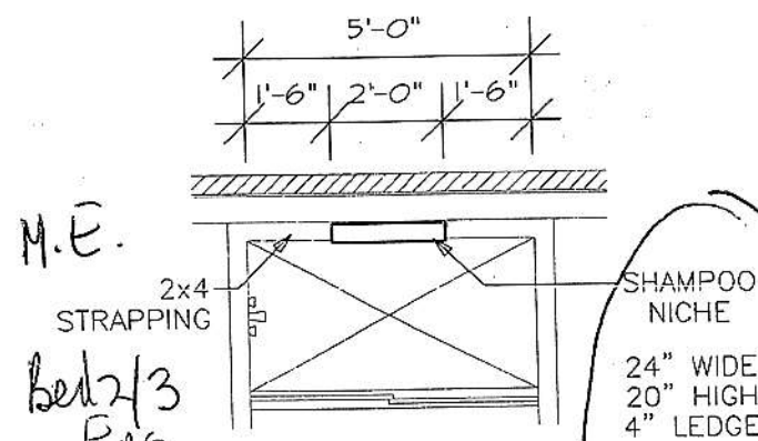
PLAN EXTERIOR WALL LONG SHOWER
