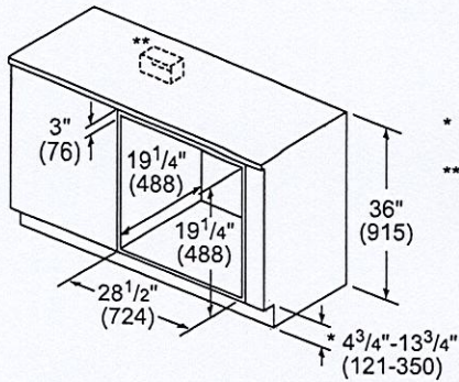
Under-counter Installation
