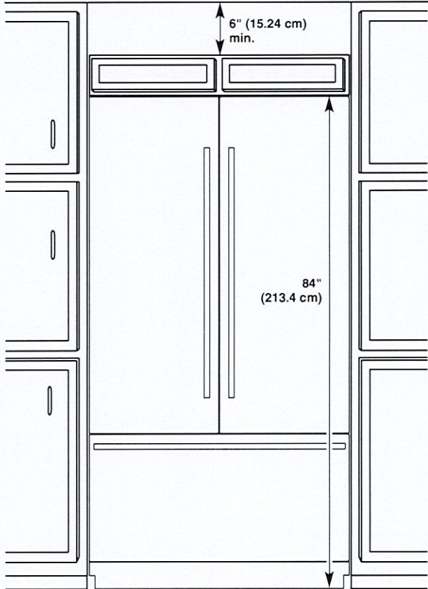
Option 2 - False Front (cabinet face only) (all models)
