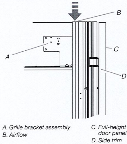
Top Grille - Side View
