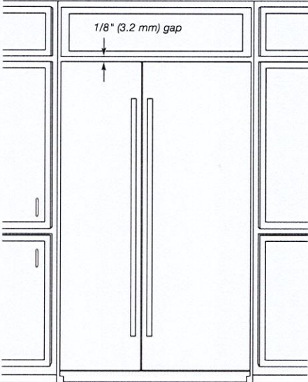
Option 3 - Closed Soffit
