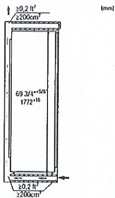
KS7793D, FNS7794E, side view (installation drawings) (US)
