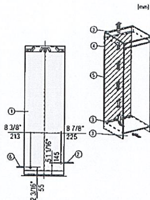
FNS7794E, installation (*footnote) (installation drawings) (US)
