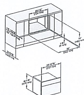
installation 30 inch Flush inset built-under wide front BM30, installation drawing, NA
