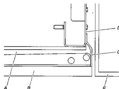
A. Refrigerator door B. Armoire-style door panel C. Side trim D. Grille bracket E. Adjacent cabinet
