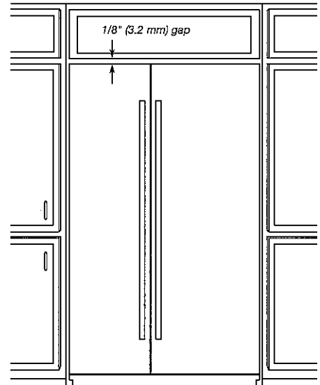
Option 3 - Closed Soffit
