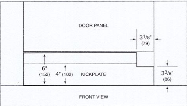
Kickplate notch
