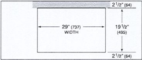
COUNTERTOP CUT-OUT
