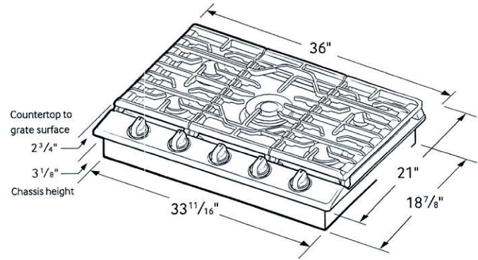
Cooktop Dimensions
