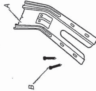
A. Anti-tip bracket B. #12 x 15/16" screws (2)
