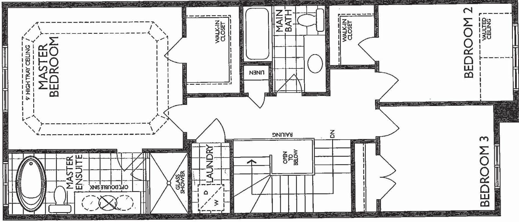
SECOND FLOOR ELEVATION A
