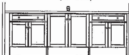
MASTER ENSUITE (2ND FLR)
