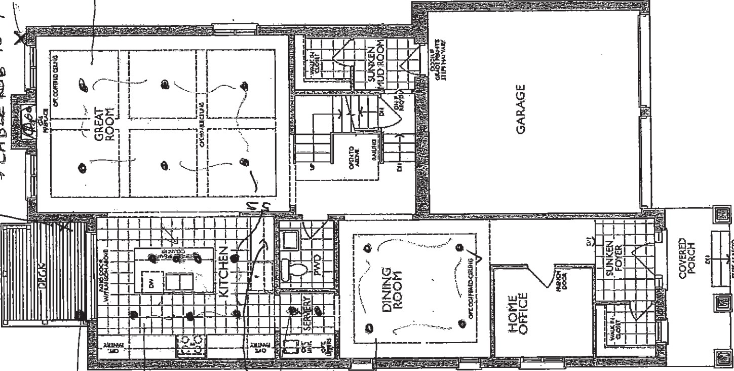
MAIN FLOOR ELEVATION A
