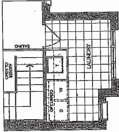
PARTIAL SECOND FLOOR WITH OPT. LAUNDRY ELEVATION B
