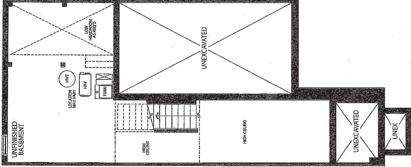
BASEMENT ELEVATION A & B
