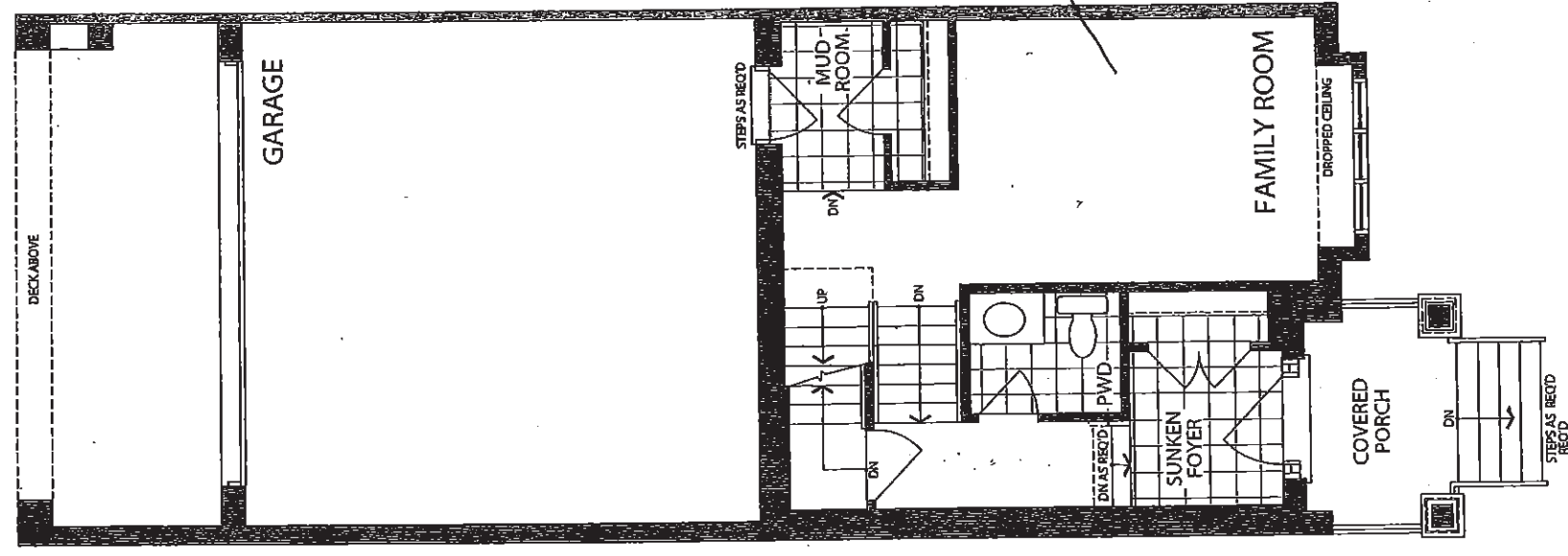
LOWER LEVEL ELEVATION A - END
