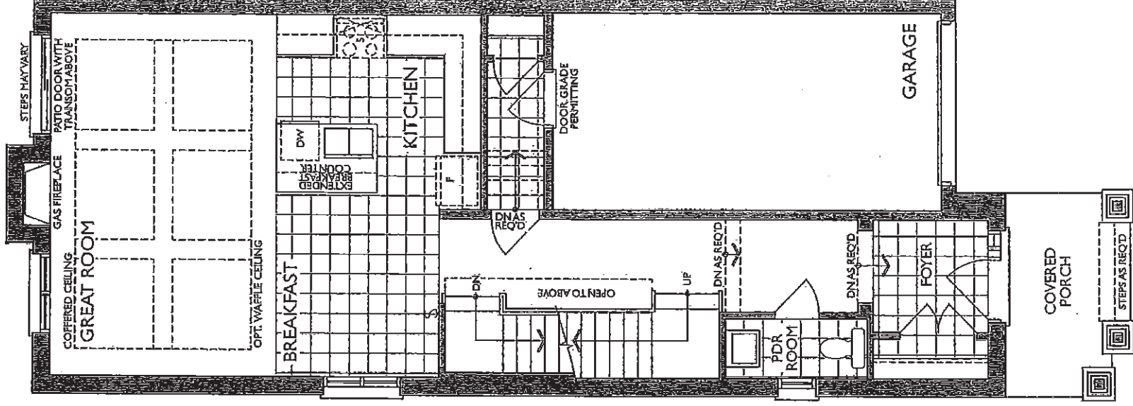
GROUND FLOOR ELEV. A
