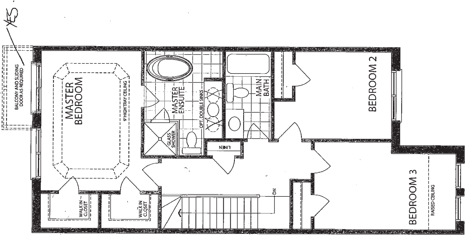
UPPER LEVEL ELEVATION B
