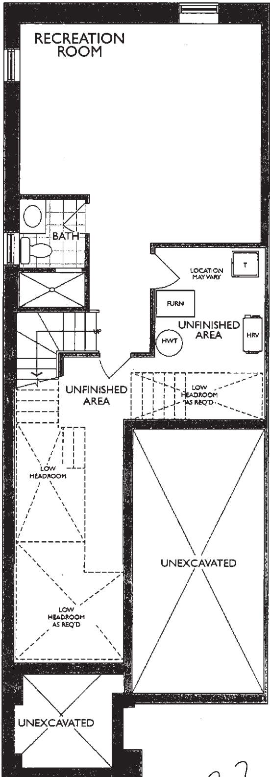
LOWER LEVEL ELEVATION B - END
