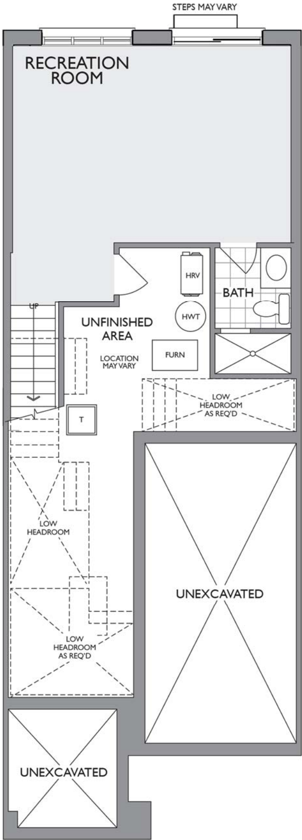
LOWER LEVEL ELEVATION A & B
