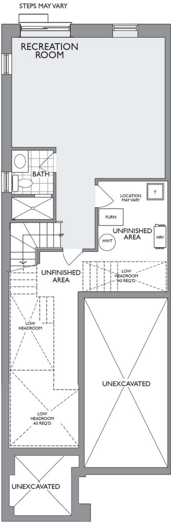
LOWER LEVEL ELEVATION B - END
