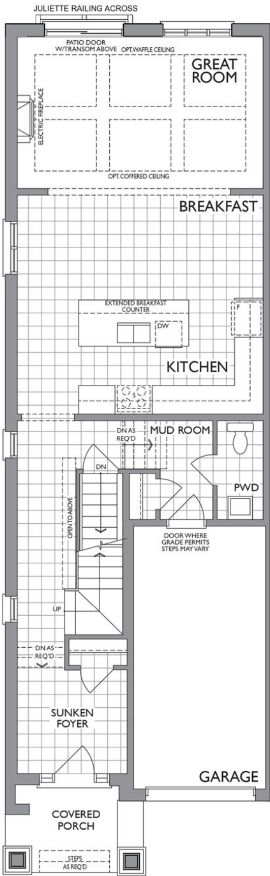
MAIN FLOOR ELEVATION A
