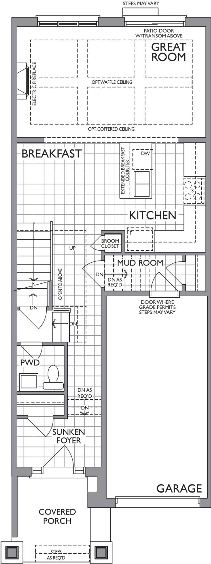
MAIN FLOOR ELEVATION A
